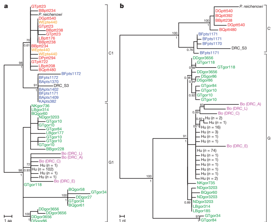
Figure 3 | Evolutionary relationships of ape and human Plasmodium parasites in mitochondrial coding and non-coding regions. a, b , Phylogenetic trees of SGA-derived mitochondrial CYTB, COXI and COXIII proteins (980 amino acids; a ) and non-overlapping nucleotide sequences (2,501 bp; b ) of the closest chimpanzee (C1) and gorilla (G1) relatives of human P. falciparum (see Supplementary Fig. 1a for the position of the corresponding 3.4-kb and 3.3-kb SGA amplicons). Plasmodium sequences are labelled and colour-coded as in Fig. 2, except for sequences derived from captive
